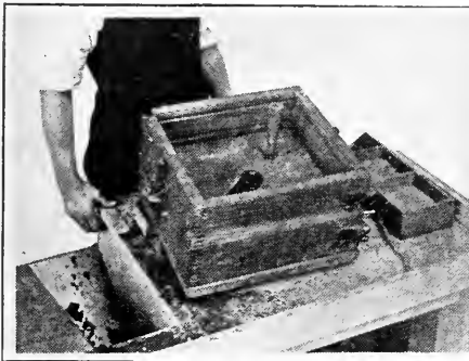
FIG. 506. COPE PLACED AND SPRUE PIN SET.
